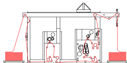
Line of Tigering machine and Polishing-Shearing machine.
