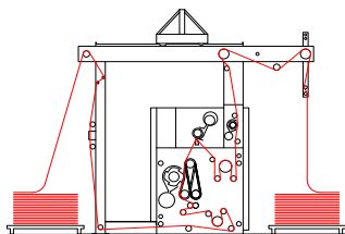
Combined Polishing and Shearing machine.
