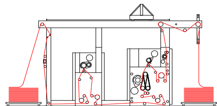
Line of Tigering machine and Polishing-Shearing machine.
