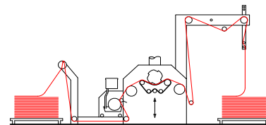
Polishing machine for wool and cashmere fabrics.
