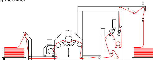
Line of Polishing and shearing machine.
