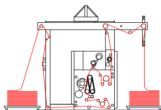
Combined Polishing and Shearing machine.
